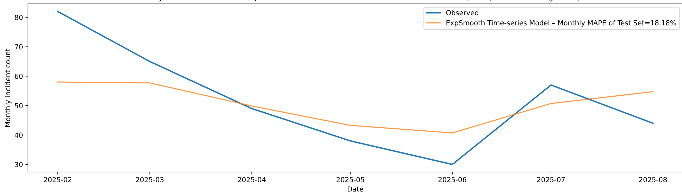
Monthly Traffic Incidents in Yeşildere Street: Best Time-series Model vs Observed (TEST, Feb 2025-Aug 2025)
