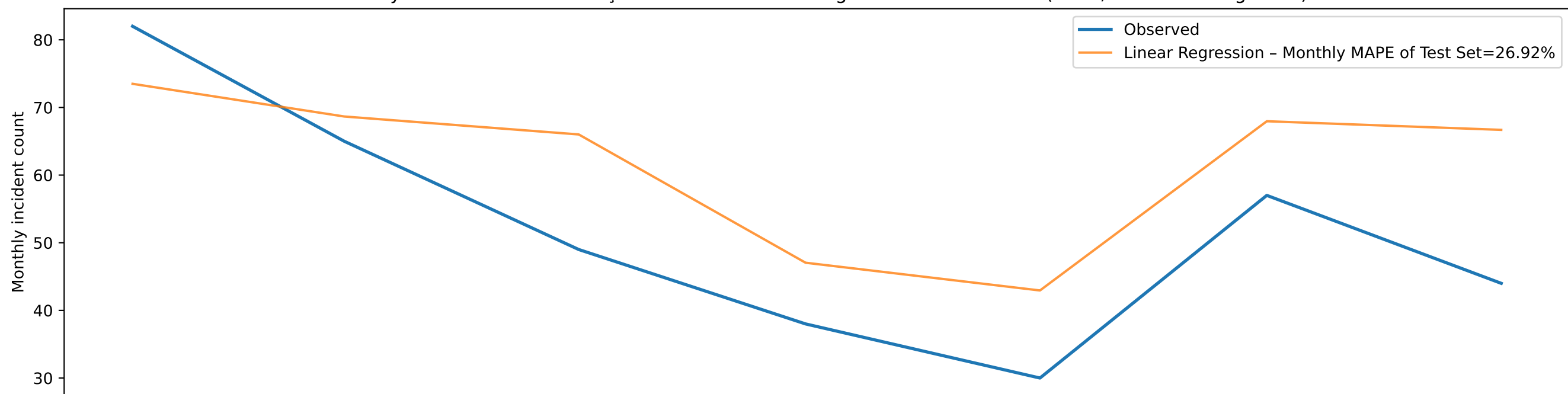
Monthly Traffic Incidents in Yeşildere Street: Best Time-series Model vs Observed (TEST, Feb 2025-Aug 2025)
